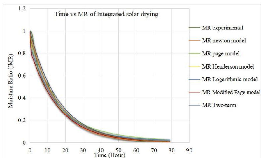
Figure 7. Time vs MR of Integrated solar drying.
