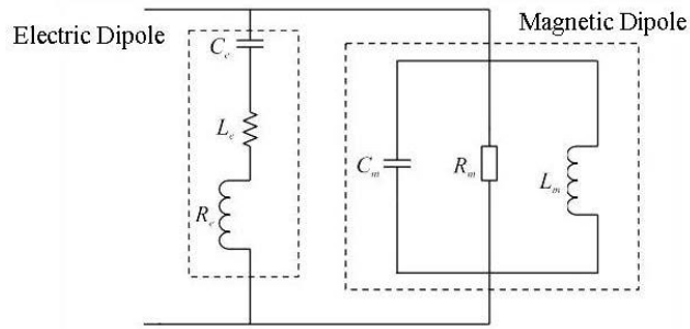
Figure 4. Equivalent circuit of the magnetoelectric dipole
